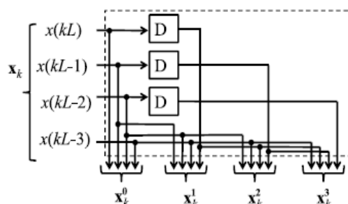
Fig. 2. Register Unit
